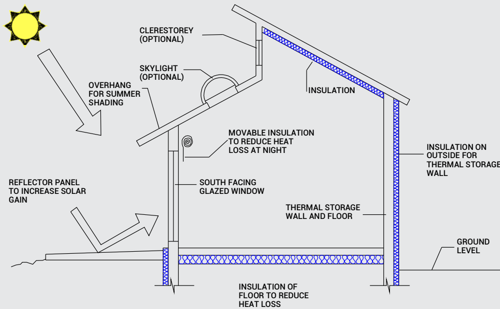
FIGURE 30. Direct solar gain system. (Image from Nayak and Prajapati, 2006) 136
