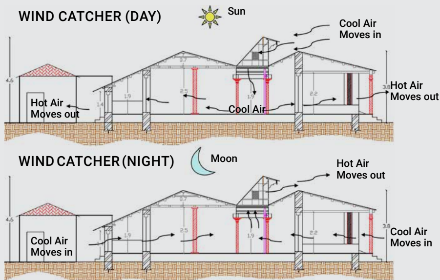
FIGURE 20. Daily energy management in traditional building in Nagapattinam (Image from Priya, Sundararaja, 2012) 124
