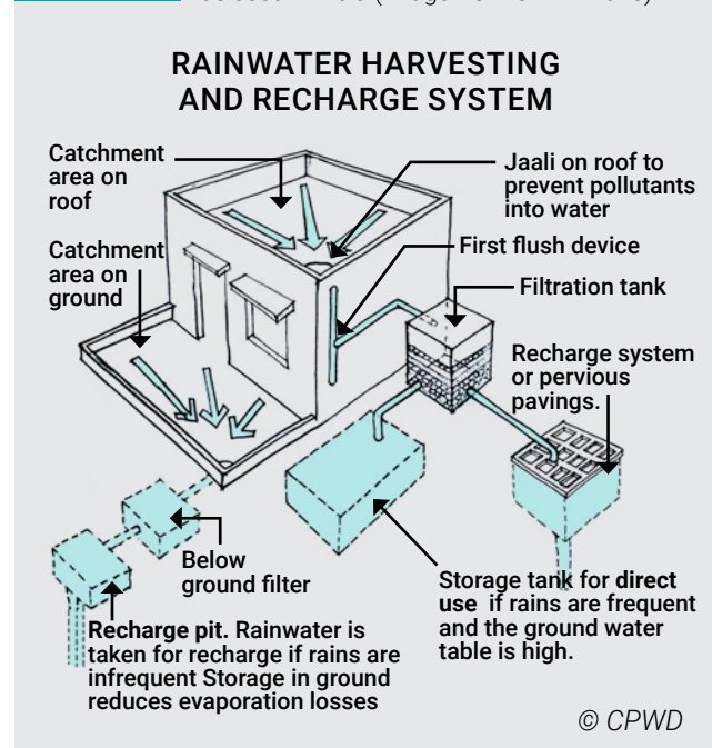
FIGURE 33. Rainwater harvesting and recharge system as used in India (Image from CPWD 2013) 122
