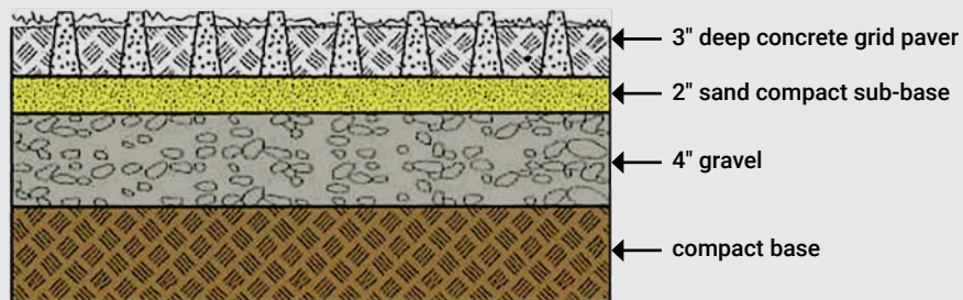
FIGURE 35. Lattice unit grids for storm run-off control, pedestrian pathways and soil conservation (Image from: TERI, 2004). 149
