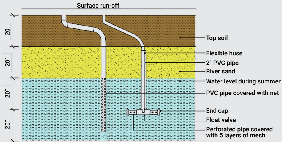
FIGURE 36. Rainwater harvesting combined with a pavement design at an interval dependent on the run-off (Image from: TERI, 2004) 149
