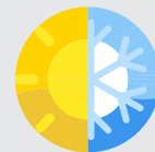
Temperate Climate
