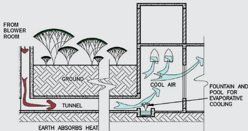
FIGURE 24. Earth air tunnel system utilizing underground temperature to cool (Kamal 2012) 127
