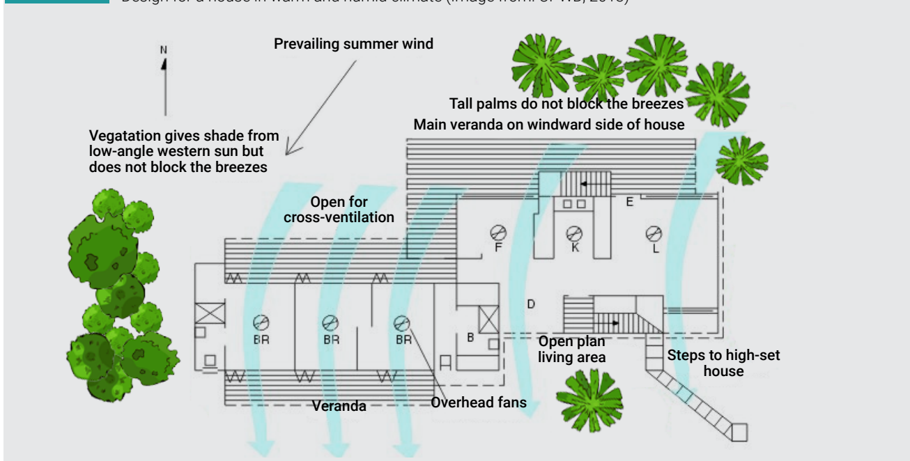
FIGURE 18. Design for a house in warm and humid climate (Image from: CPWD, 2013) 122
