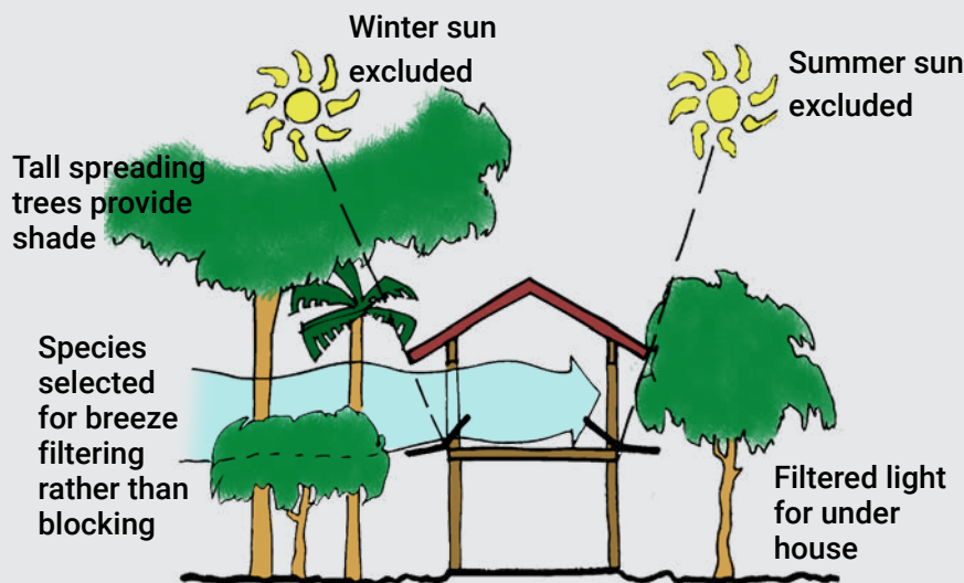
FIGURE 19. Hot and humid climate, maximising higher elevation and vegetation for cooling breezes (Image from McGee, Reardon) 123
