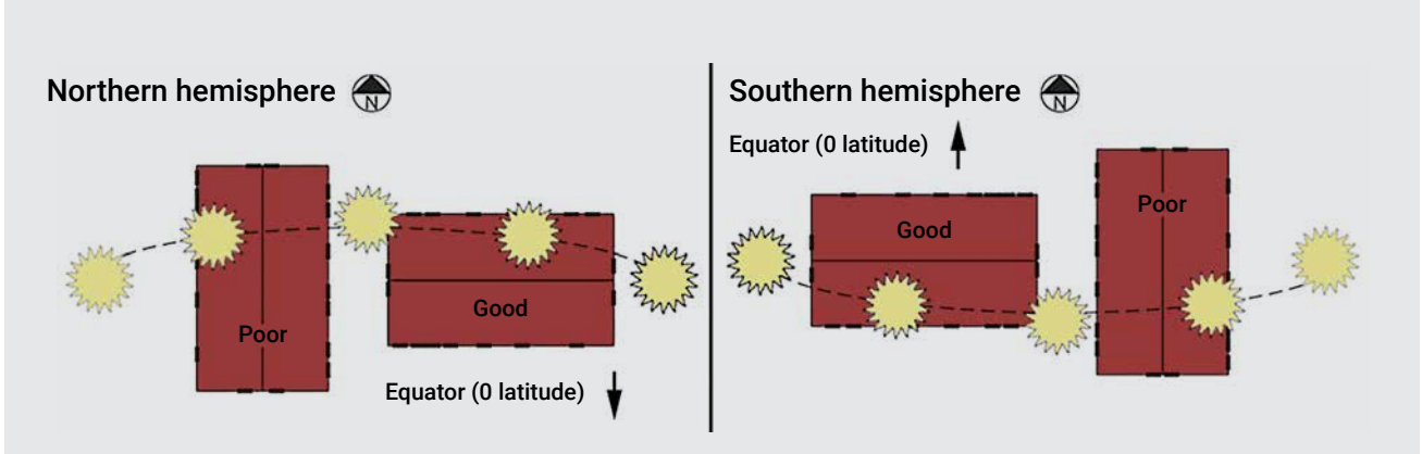
FIGURE 14. Ideal orientation of a building in both hemispheres (Image adapted from: Rupperta, Millera 2015) 117
