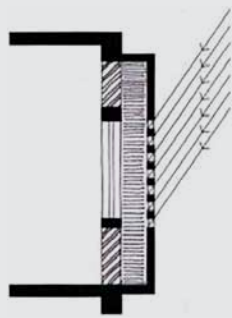
FIGURE 26. Windows and shading strategies for hot and dry climate regions (Image from CPWD 2013). 122
