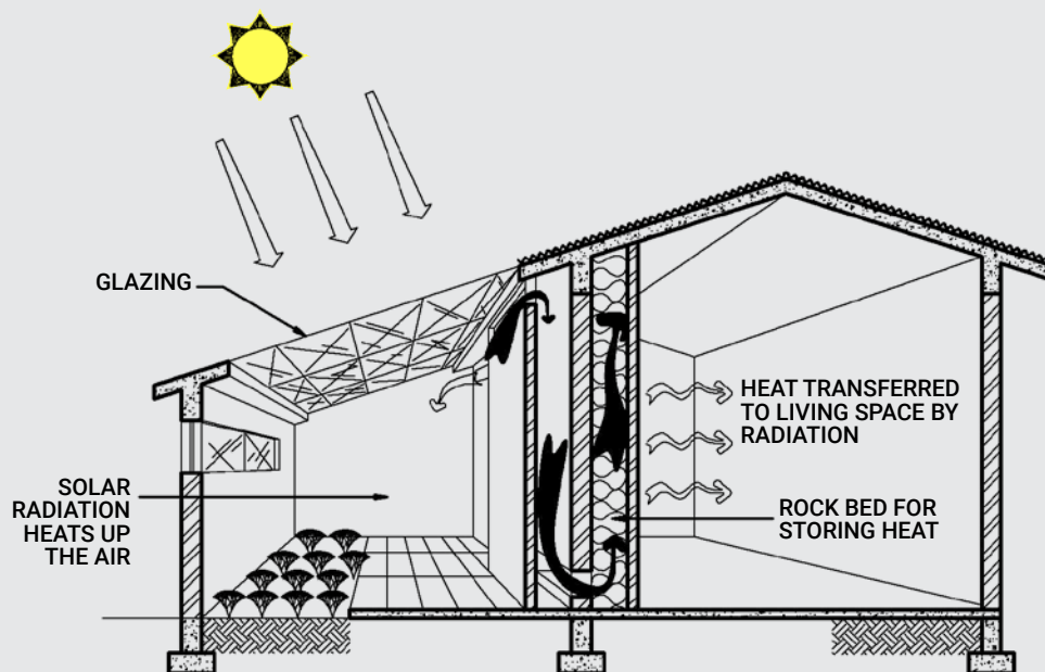
FIGURE 31. Solarium with Trombe wall as used in High Mountain regions (Diagram from Nayak and Prajapati, 2006) 136
