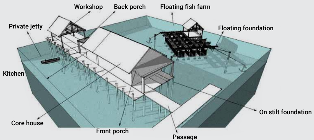
FIGURE 38. Malaysian water building design (Image from: Lai and Cheng, 2019) 152
