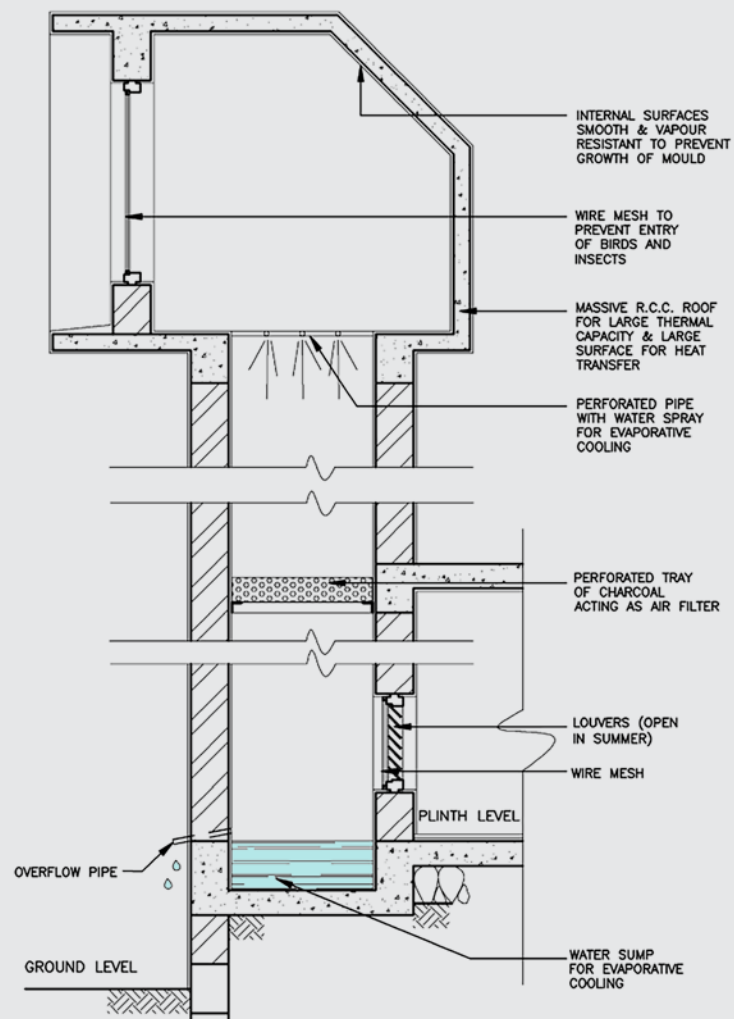
FIGURE 23. Central wind tower with water for cooling for use in hot and dry climates (Image from Kamal, 2012) 127
