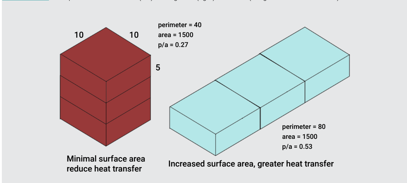
FIGURE 15. Low perimeter to area ratio (left) and high P/A (right) illustrated (Image redrawn from CLEAR). 118
